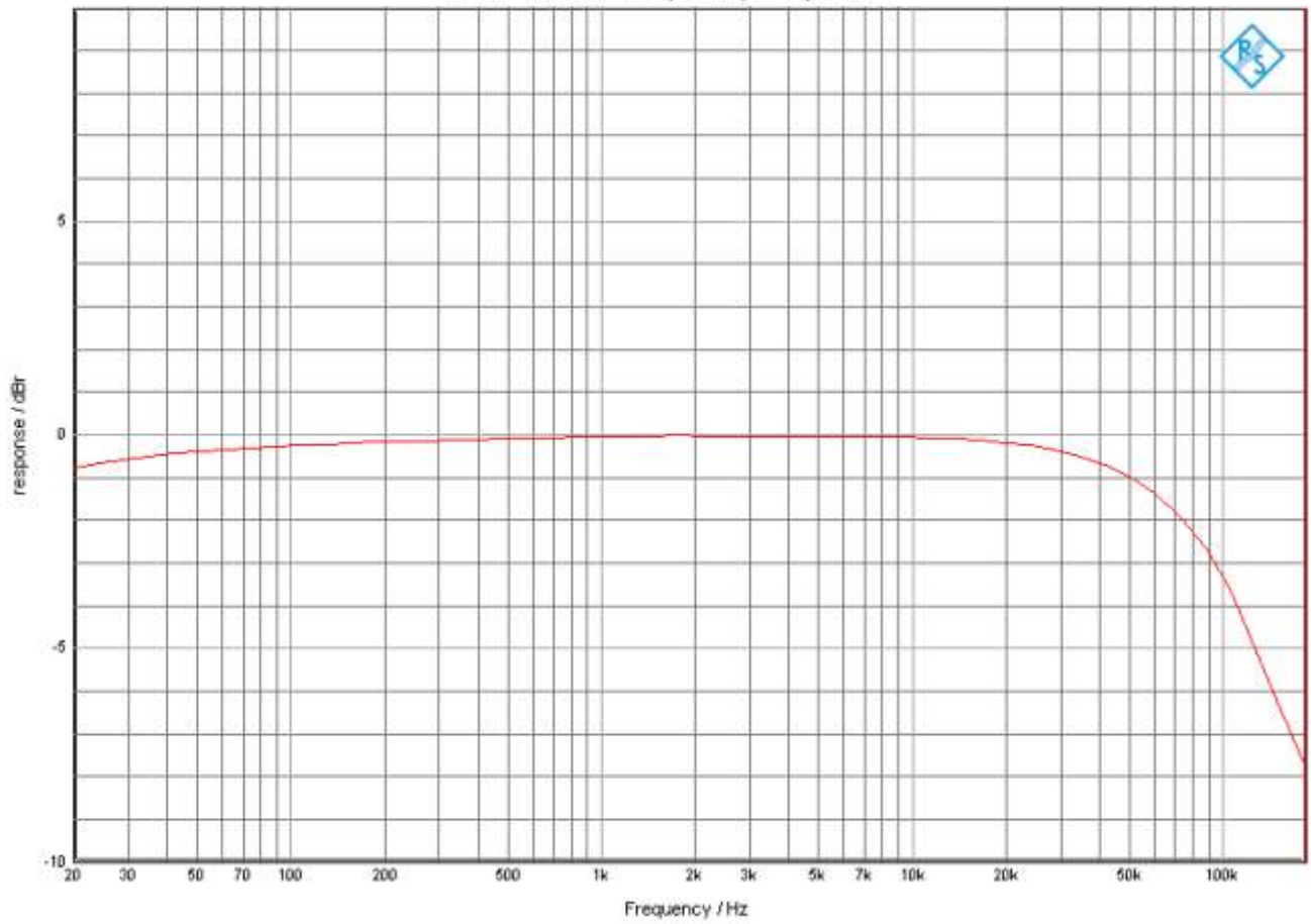
40PP4K0H - frequency response
