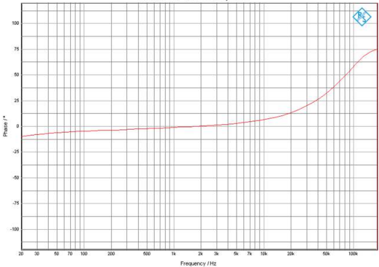
40PP4K0H - Phase response
